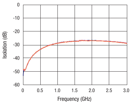
RFC to RF2 Isolation
