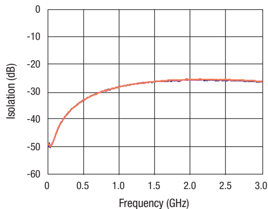
RFC to RF3 Isolation
