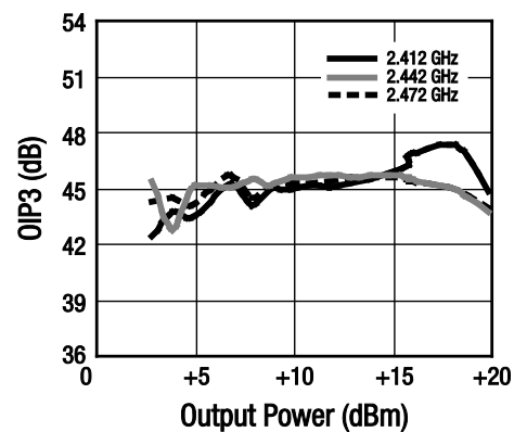
Figure 61. OIP3 vs Output Power Over Frequency
