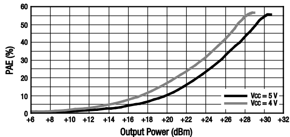
Figure 17. Output Power vs PAE Over Voltage
