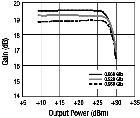
Figure 6. Gain vs Output Power Over Frequency
