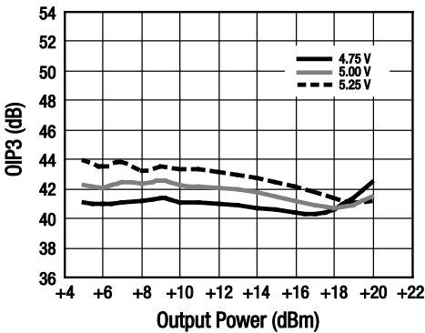
Figure 16. OIP3 vs Output Power Over Voltage
