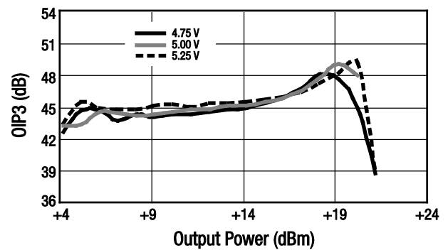
Figure 48. OIP3 vs Output Power Over Voltage
