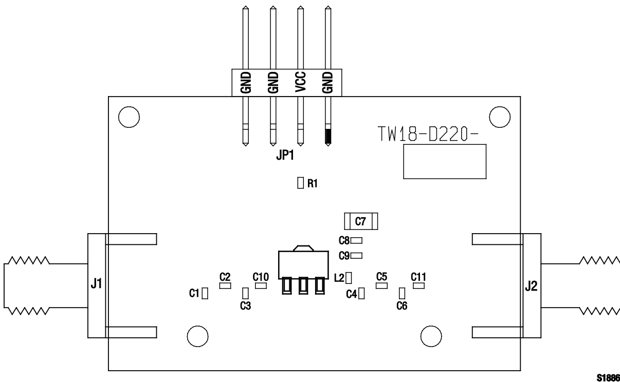
Figure 73. Evaluation Board Assembly Drawing
