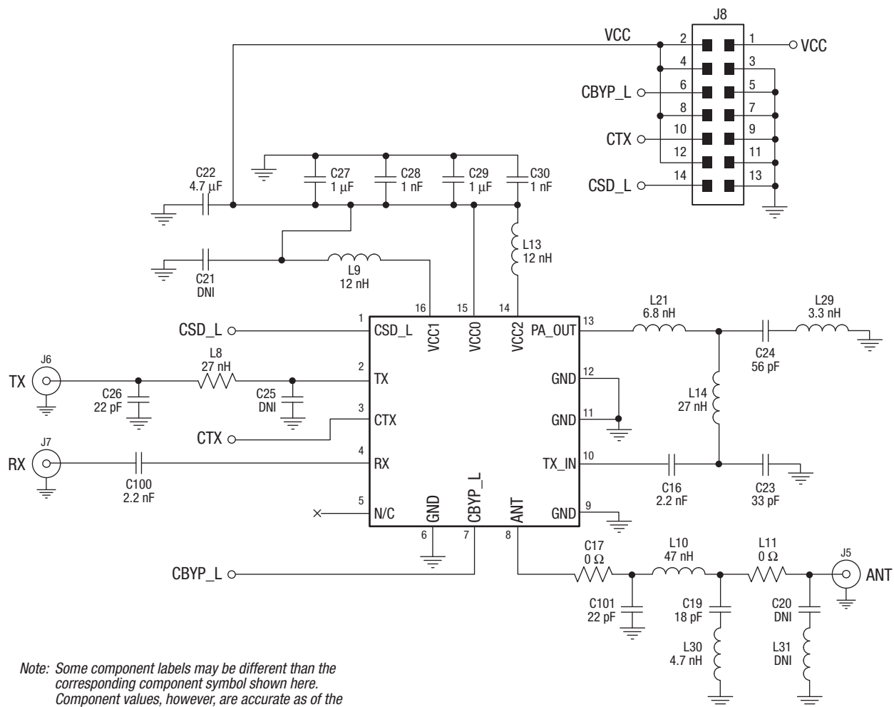
Figure 4. SKY66100-11 EK-2 Evaluation Board Schematic (+27 dBm)
