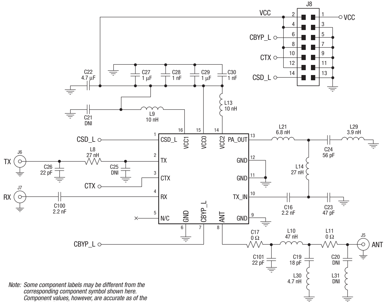
Figure 3. SKY66100-11 EK-1 Evaluation Board Schematic (+24 dBm)
