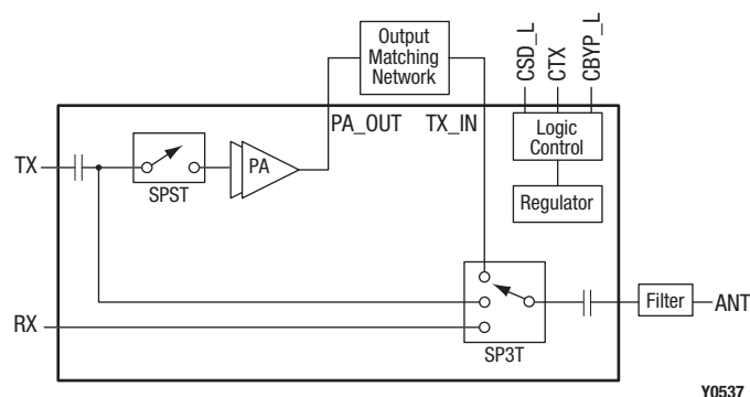
Figure 1. SKY66100-11 FEM Block Diagram
