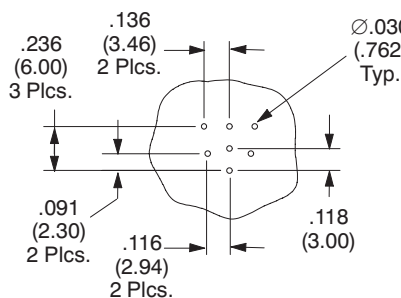
PC Board Layout for D02EEB706FD21TABH
