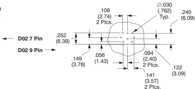
PC Board Layout for D02EEB906FD21TABH
