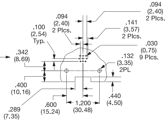
PC Board Layout for D02EEB906FB24TABH
