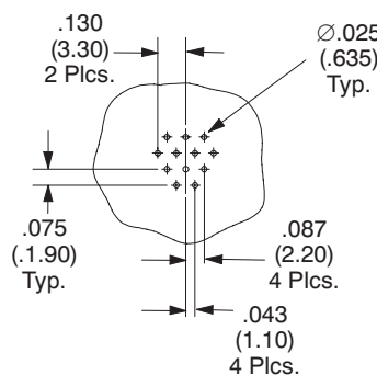
PC Board Layout for D02EEB125FD21TABH
