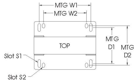
Mounting Dimensions
