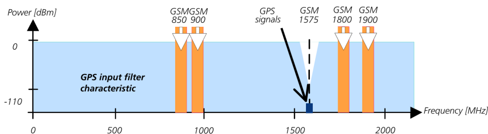
Figure 15: Out-band interference signals
