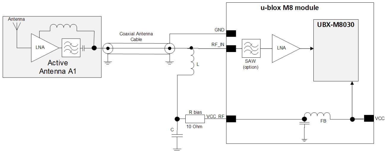
Figure 8: Active antenna design, external supply from VCC_RF (for exact pin orientation see the NEO-M8P Data sheet [1])
