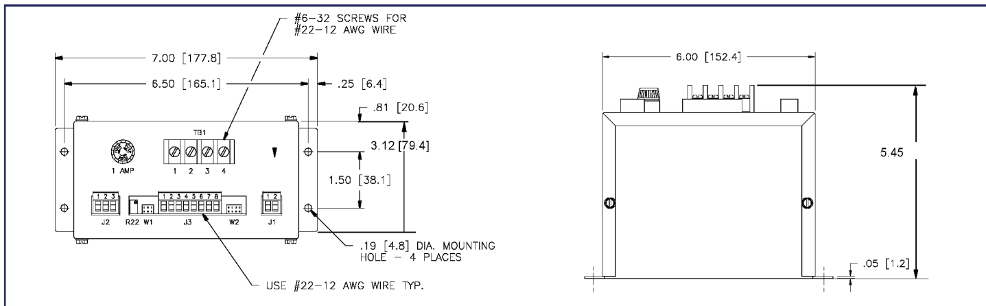
FRC-20 Dimensions
