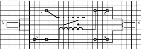
Pin # 5 must be positive for Form B version
