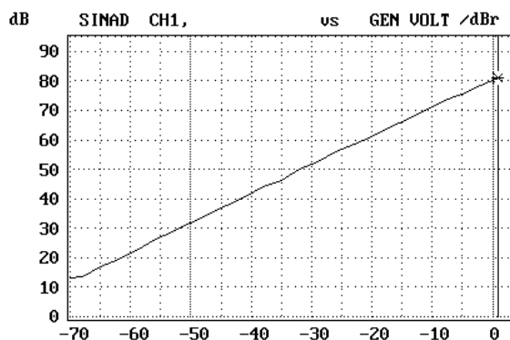
Figure 3. Voice RX performance S/(N+THD) [dB] versus signal amplitude [dBm0] with 8Ω output load VCC=2.7V, F_s=8\text{kHz}
