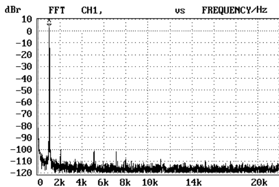
Figure 1. Stereo DAC performance FFT audio mode (8192 points). Full scale input/output sinewave at 1 kHz (+3dB) VCC=2.7V, F_s=48\text{kHz} , 18 bits input word.
