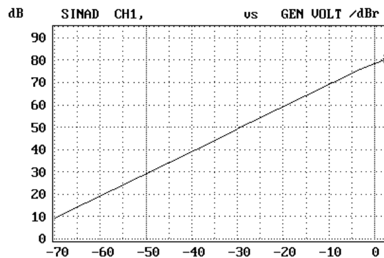
Figure 4. Voice TX performance S/(N+THD) versus signal amplitude VCC=2.7V, F_s=8\text{kHz}
