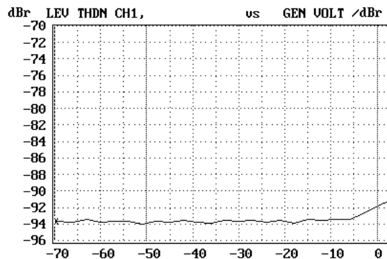
Figure 2. Stereo DAC performance Dynamic range: Noise + THD [dB] versus signal amplitude [dBm0] VCC=2.7V, F_s=48\text{kHz} , 18 bits input word.
