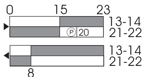
Switching diagram
