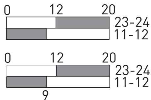
Switching diagram
