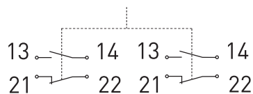
Contact diagram
