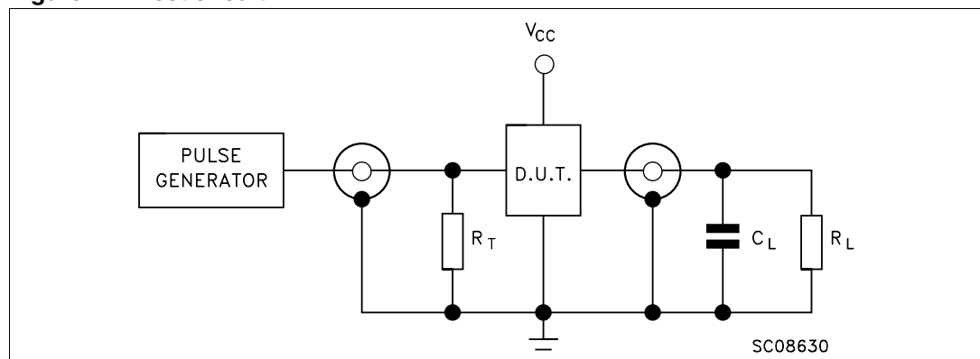
Figure 4. Test circuit
