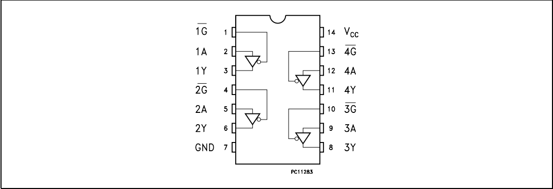
Figure 3. Pin connections (top through view)
