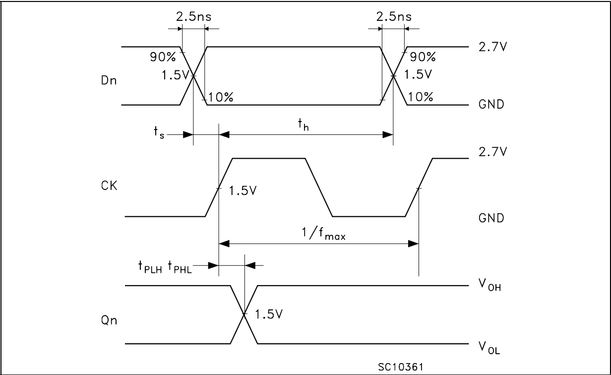
Figure 5: Waveform - Propagation Delays, Setup And Hold Times, Maximum CK Frequency ( f=1\text{MHz} ; 50% duty cycle)
