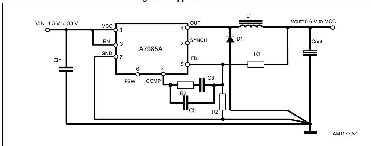
Figure 1. Application circuit
