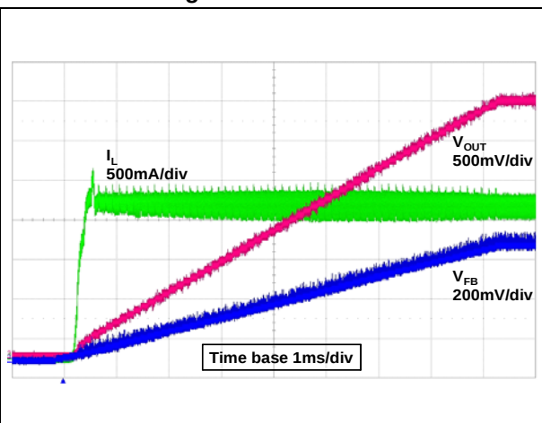
Figure 31. Soft-start
