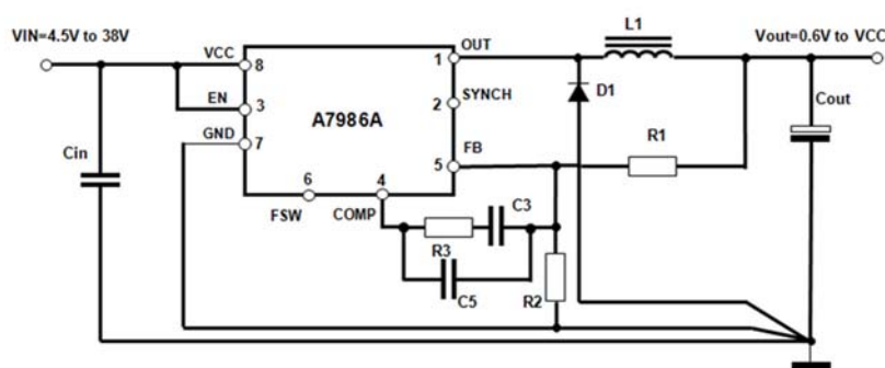
Figure 1. Application circuit
