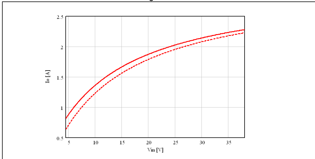
Figure 35. Maximum output current according to max. DC switch current (3.0 A): V O =12 V
