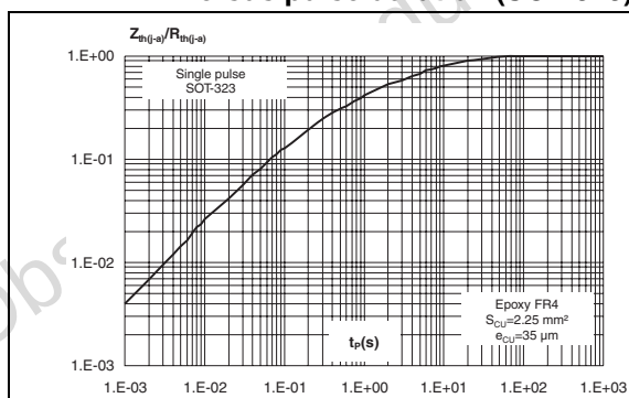
Figure 5. Relative variation of thermal impedance junction to ambient versus pulse duration (SOT-323)
