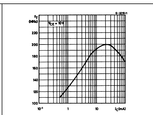
Figure 4. Transition frequency
