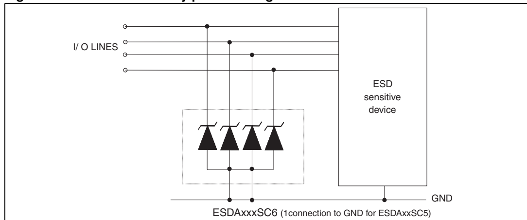
Figure 10. ESDAxxSCx array protection against ESD
