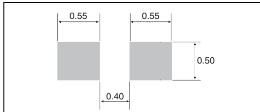
Figure 10. SOD-882 footprint (dimensions in mm)
