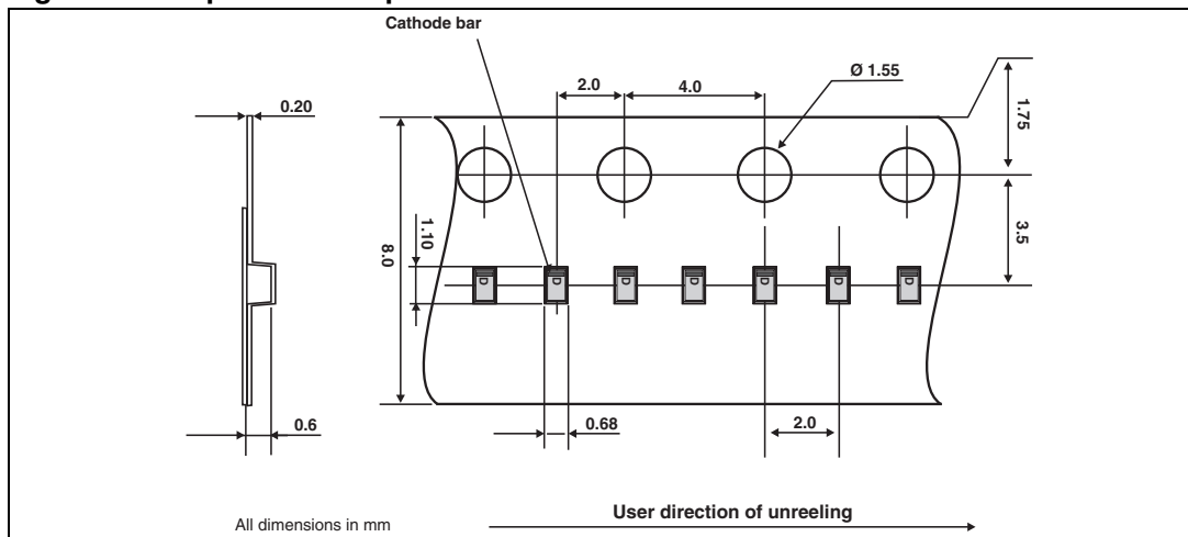
Figure 12. Tape and reel specifications
