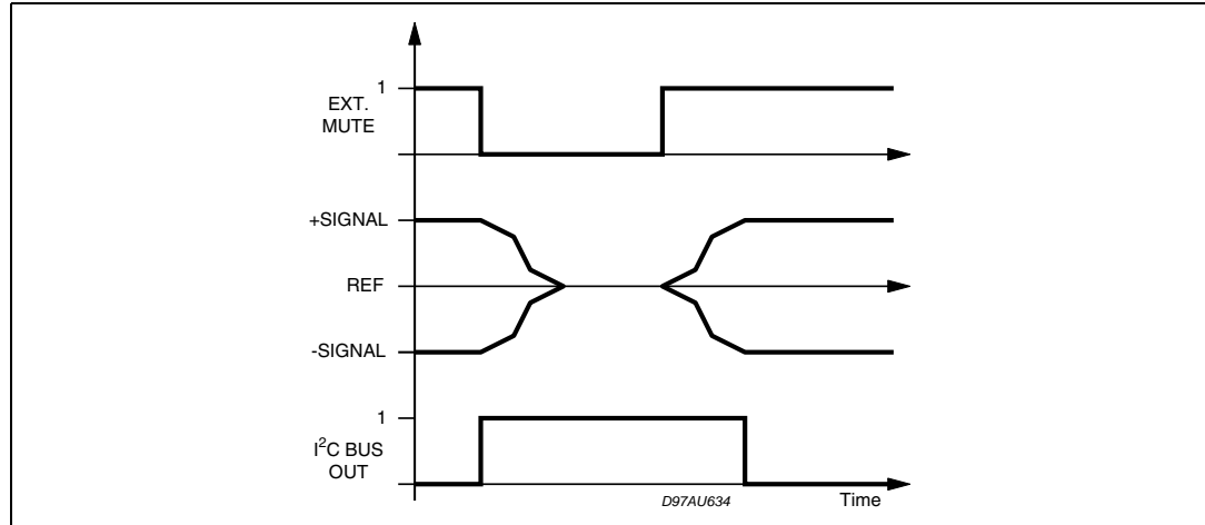
Figure 7. Softmute timing
