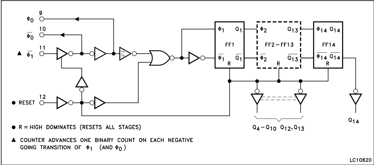
Figure 4. Logic diagram
