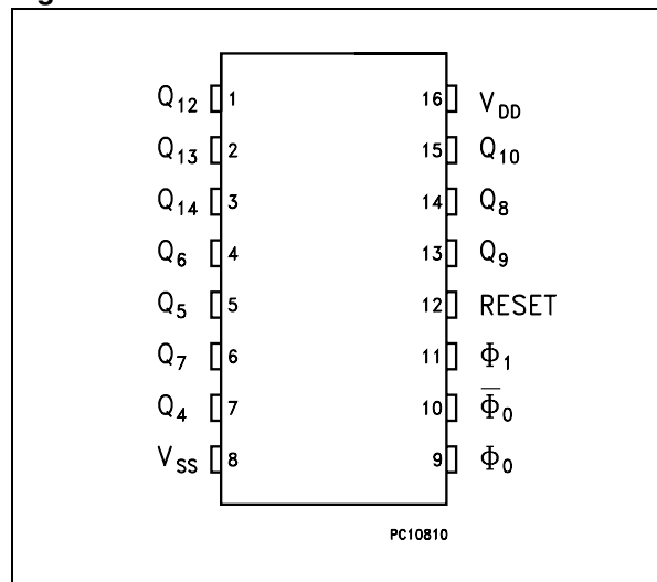
Figure 1. Pin connection
