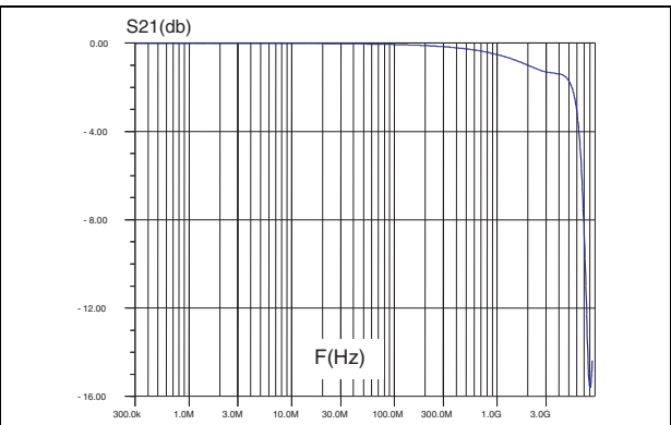
Figure 3. S21 attenuation measurement (HSP061-2P6, HSP061-2M6)
