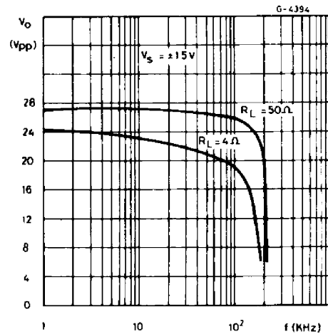
Figure 5. Large signal frequency response.
