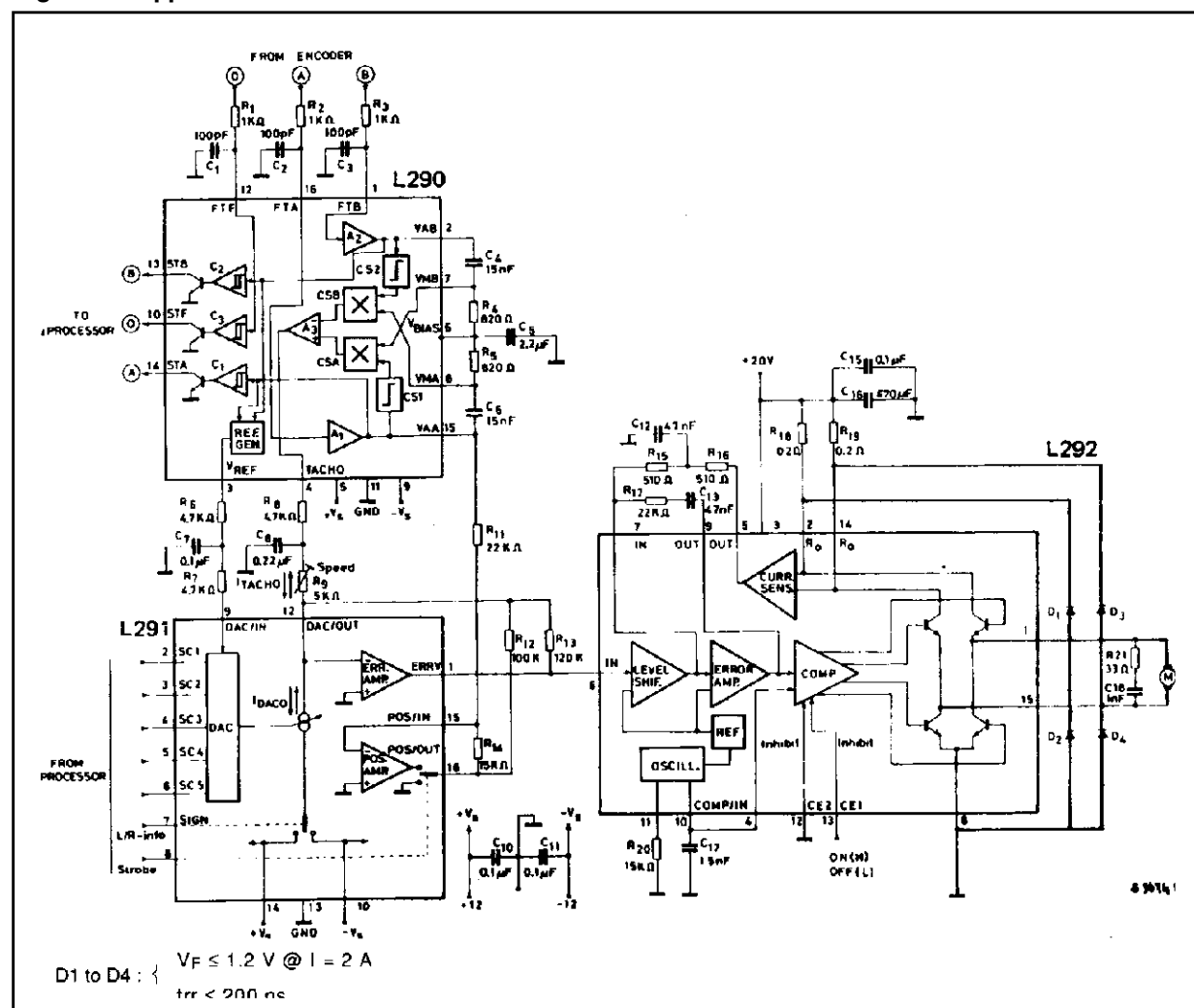
Figure 4 . Application Circuit.
