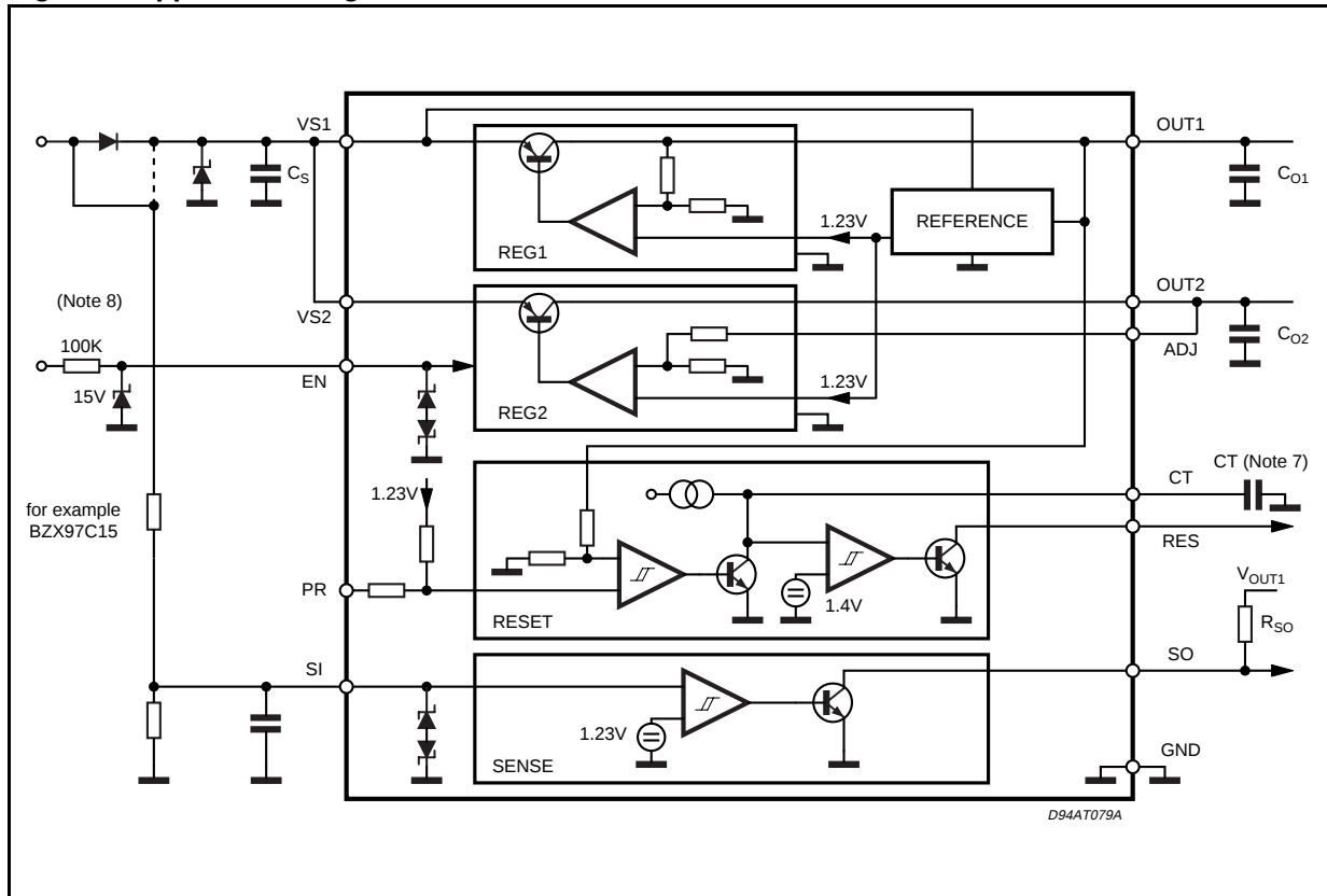
Figure 1. Application Diagram.
