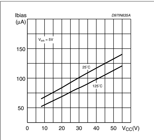
Figure 10. Stand by drain current vs. input voltage
