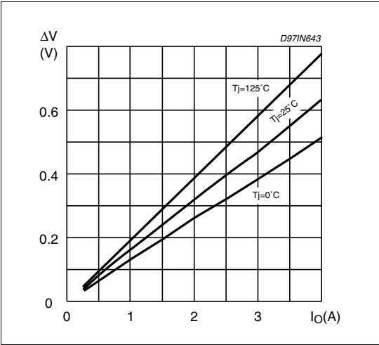
Figure 24. Dropout voltage between pin 7,8 and 2,3
