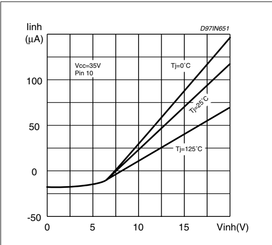
Figure 14. Inhibit current vs. inhibit voltage (pin 10)
