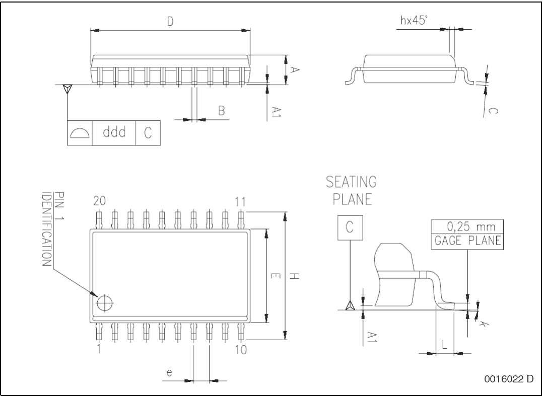
Figure 45. Package dimensions
