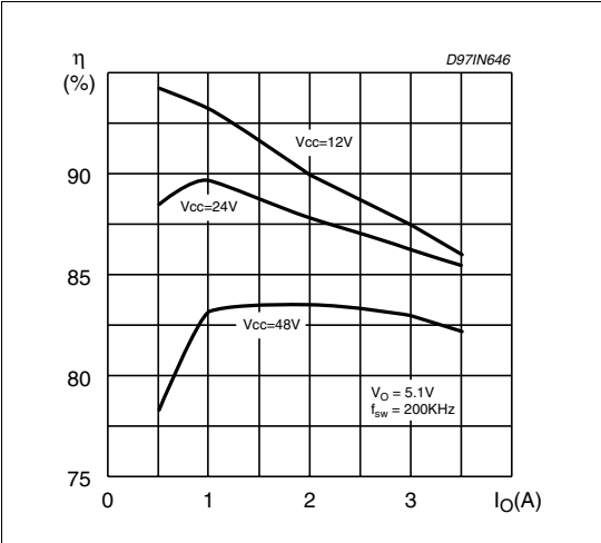
Figure 28. Efficiency vs. output current (see Figure 6)
