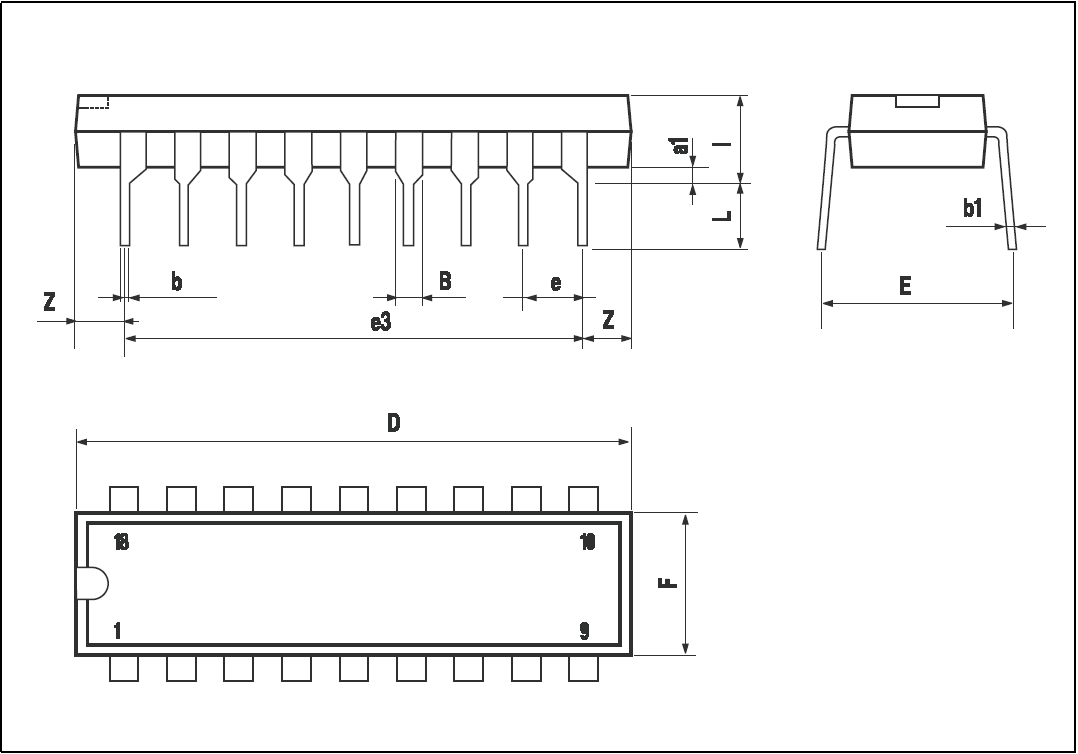
Figure 44. Package dimensions
