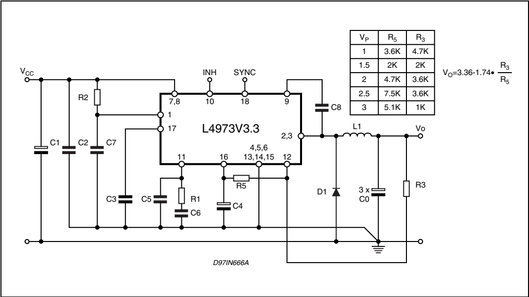
Figure 40. 3.5A at V_O < 3.3V (see part list Figure 3 )
