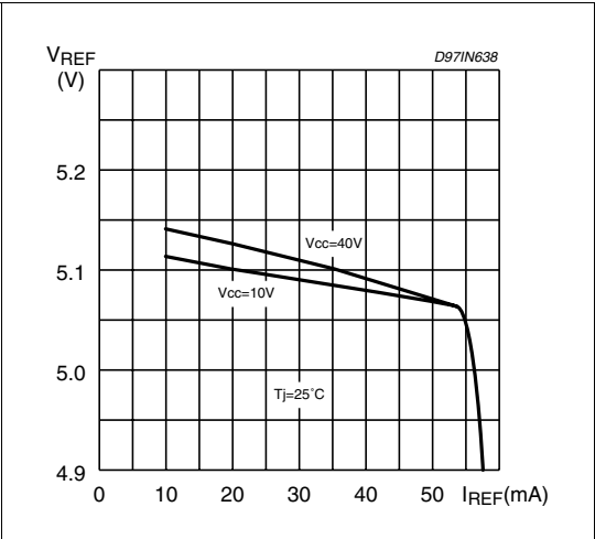
Figure 15. Line regulation (see Figure 6)
