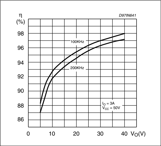
Figure 25. Efficiency vs. output voltage (see Figure 3)
