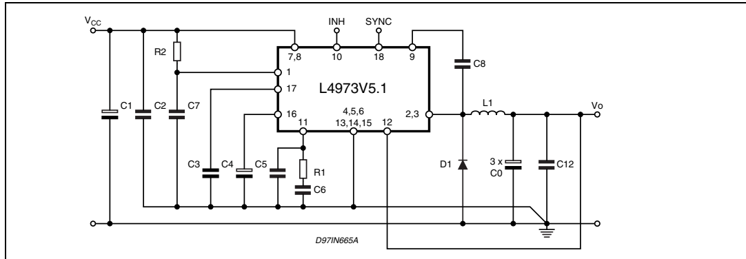
Figure 6. Application circuit (see Figure 3 part list)
