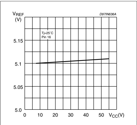
Figure 13. Reference voltage vs. input voltage (pin 16)
