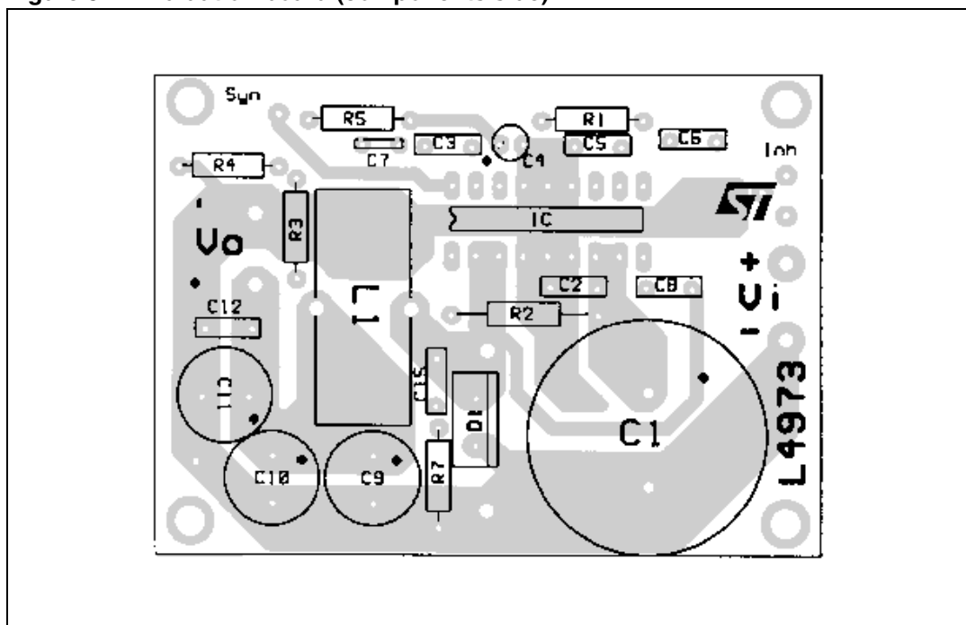
Figure 5. Evaluation board (components side)
