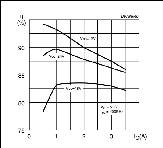
Figure 29. Efficiency vs. output current (see Figure 7)
