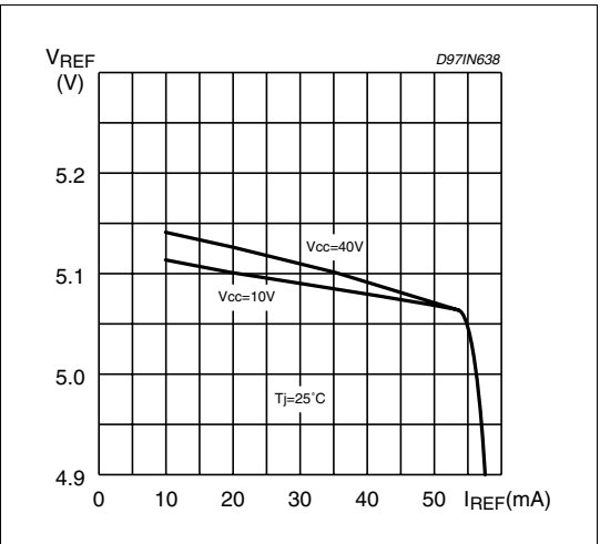
Figure 14. Reference voltage vs. reference input current
