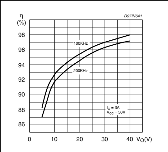
Figure 26. Efficiency vs. output voltage (see Figure 4)
