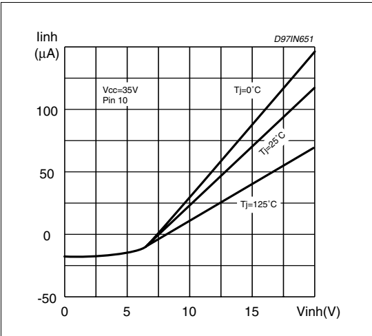
Figure 15. Inhibit current vs. inhibit voltage (pin 10)
