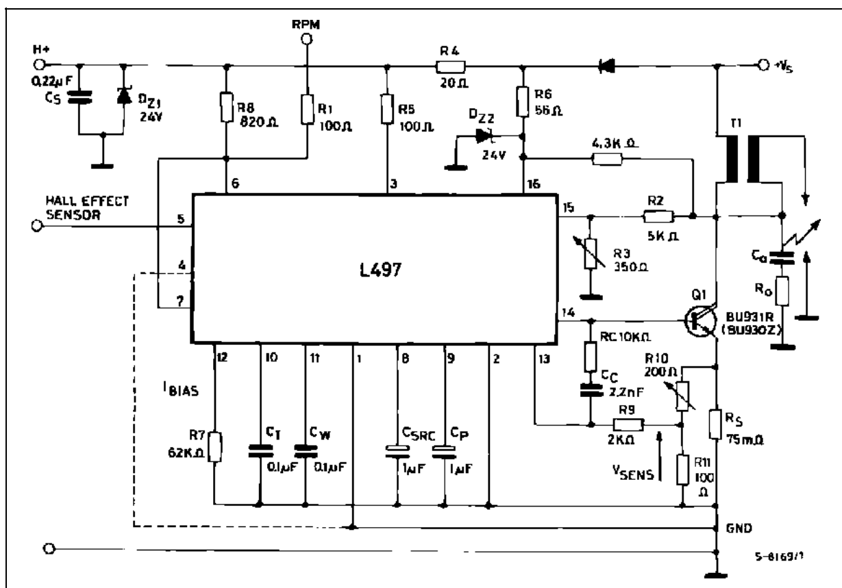
Figure 4 : Application Circuit.
