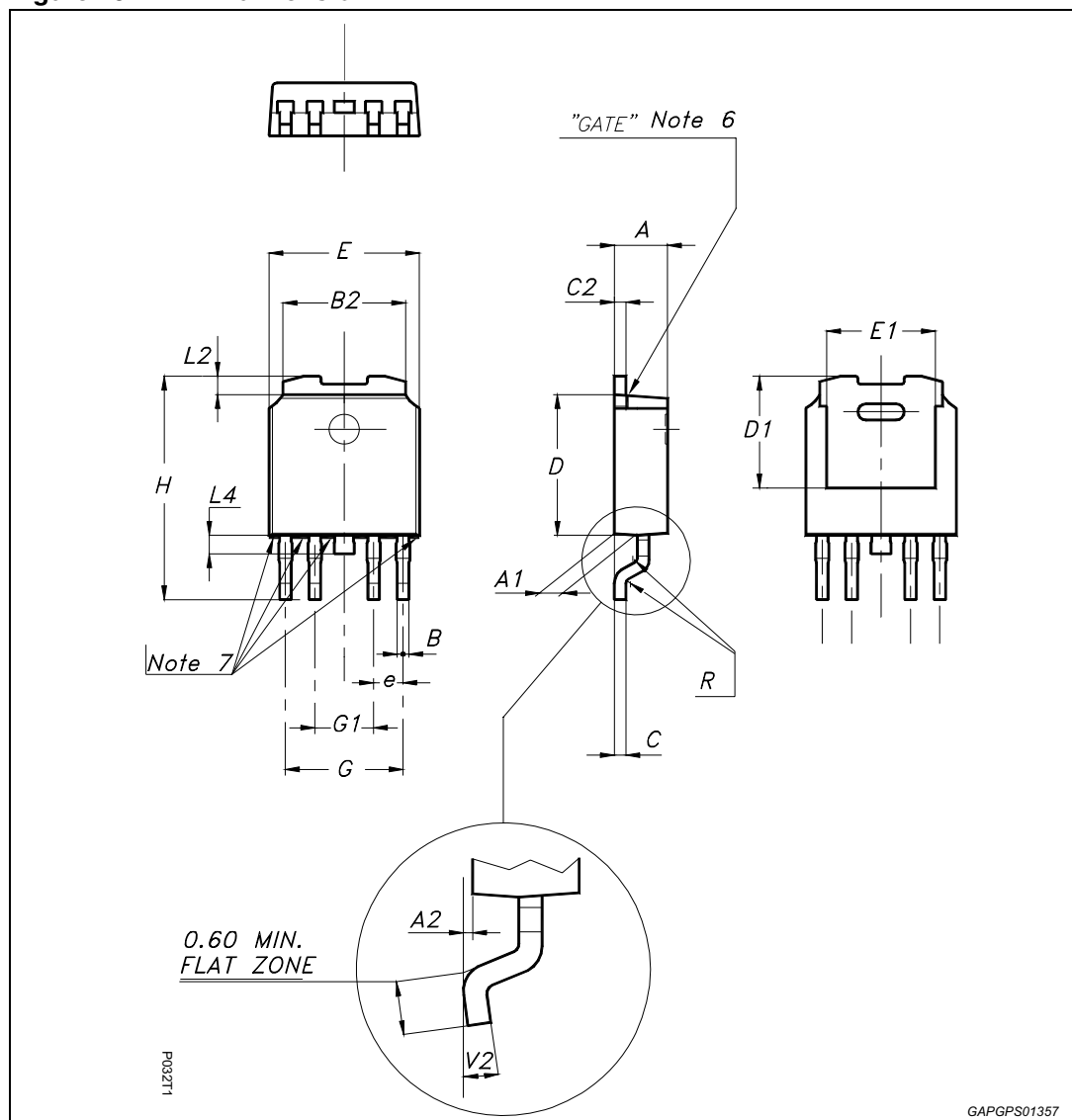
Figure 26. PPAK dimension
