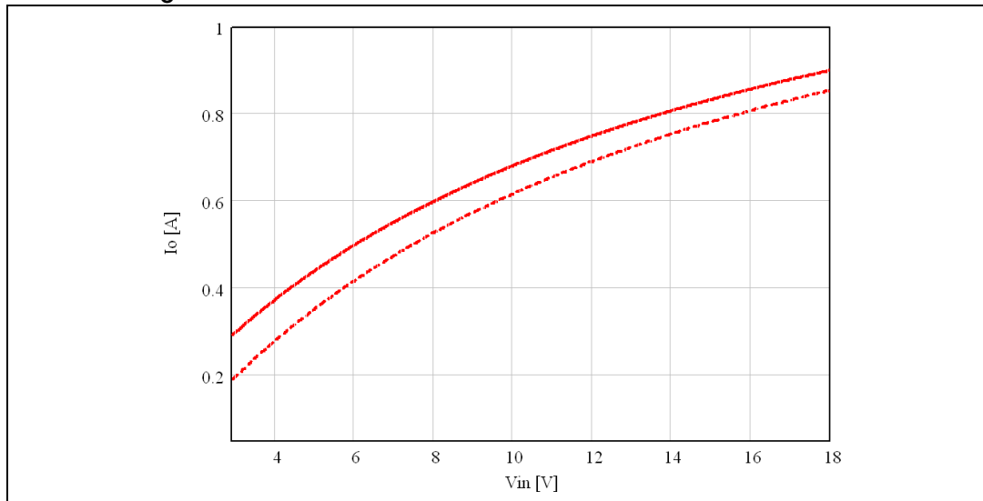
Figure 34. Maximum output current according to max DC switch current (1.5 A): V_O = 12\text{ V}
