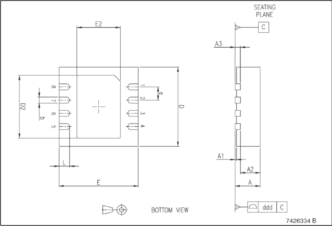
Figure 37. Package dimensions
