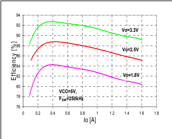
Figure 26. Efficiency vs. output current
