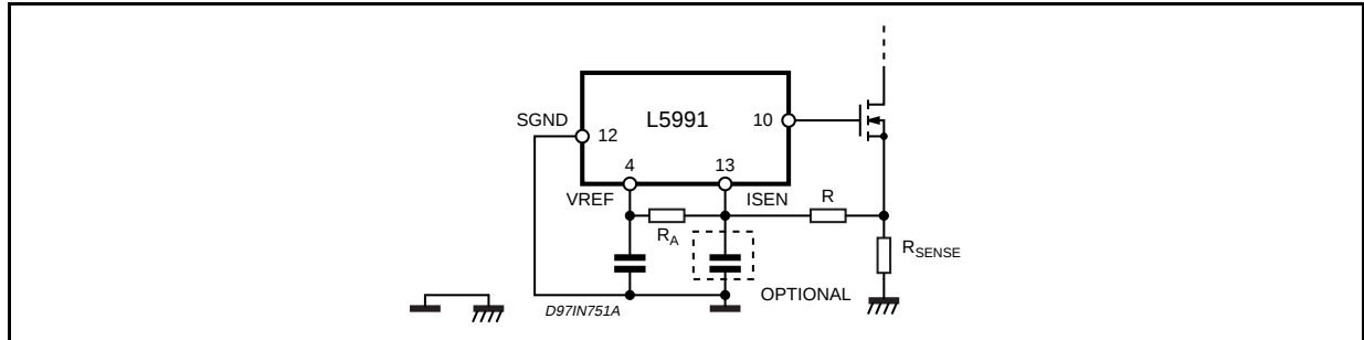
Figure 36. Isolated MOSFET Drive &amp; Current Transformer Sensing in 2-switch Topologies.
