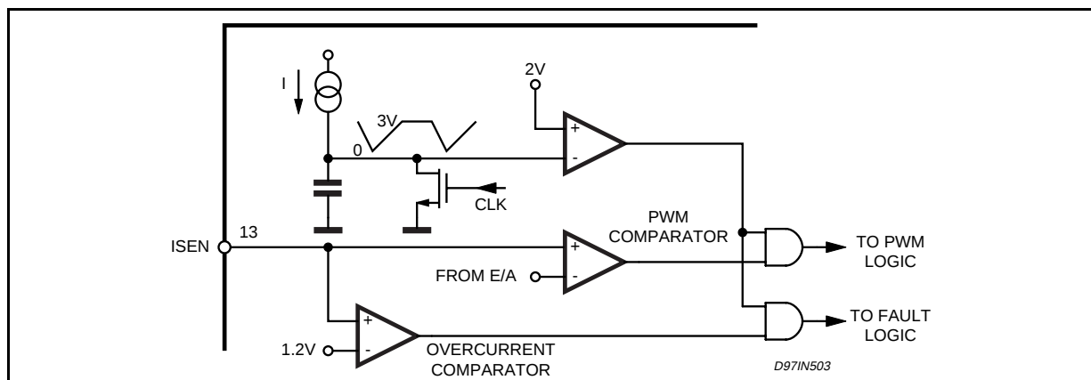
Figure 29. Internal LEB.
