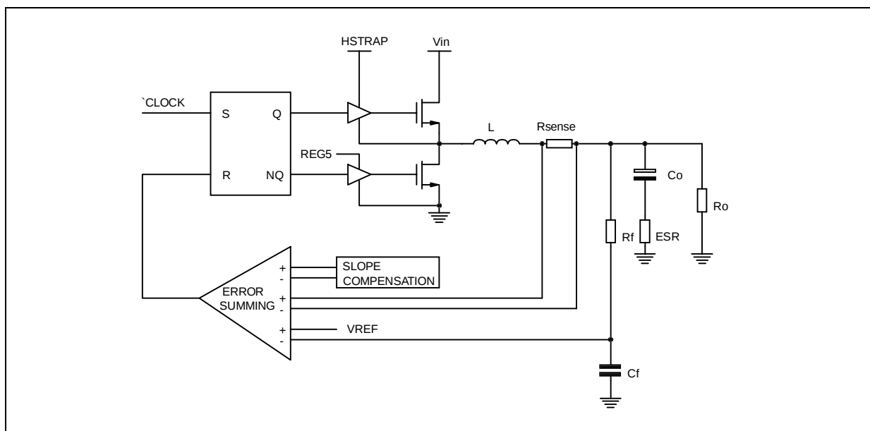
Figure 3. Control loop.
