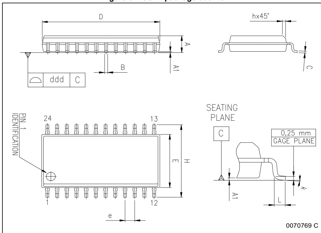
Figure 37. SO24 package outline
