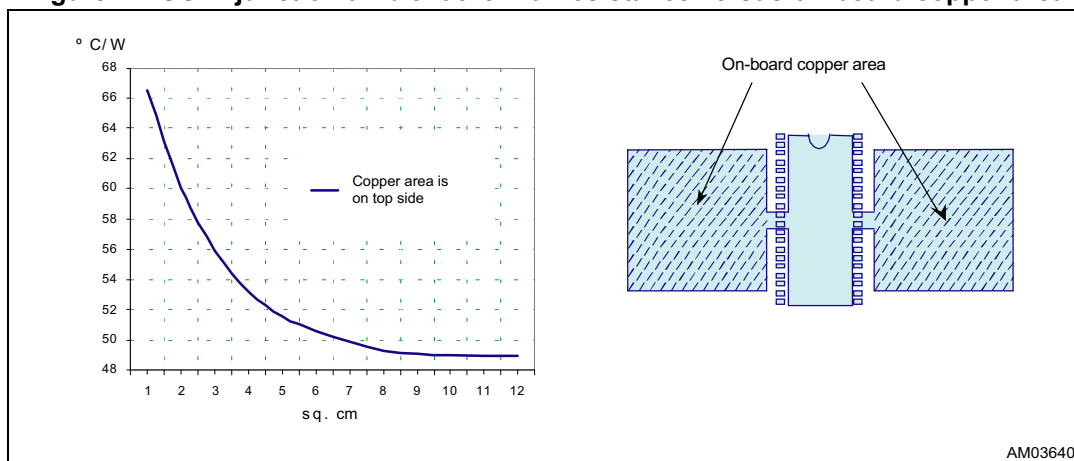
Figure 27. SO24 junction ambient thermal resistance versus on-board copper area
