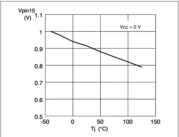
Figure 29. UVLO saturation vs T_J
