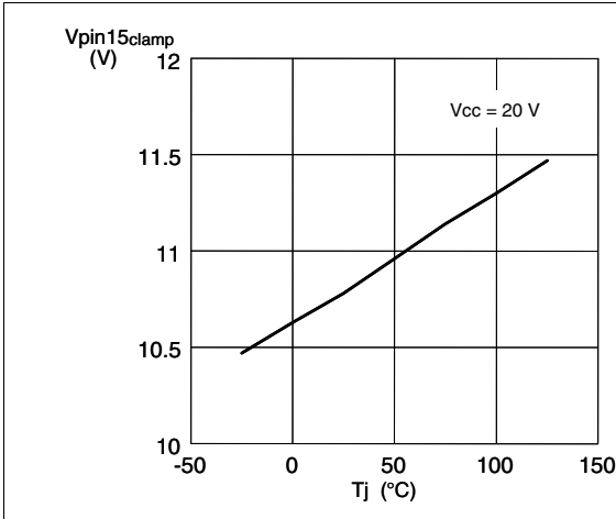
Figure 32. Gate-drive clamp vs T_J
