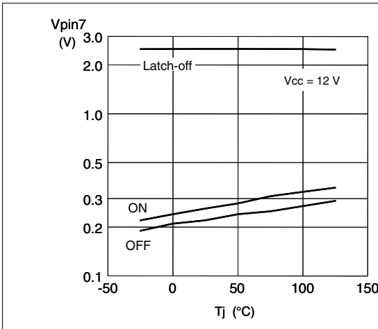
Figure 28. PFC_OK thresholds vs T_J
