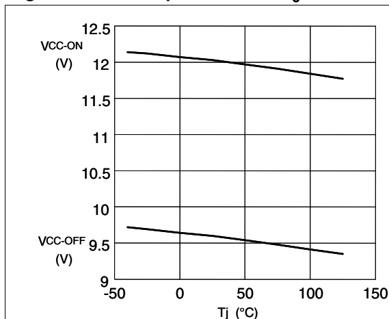
Figure 8. Start-up & UVLO vs T_j
