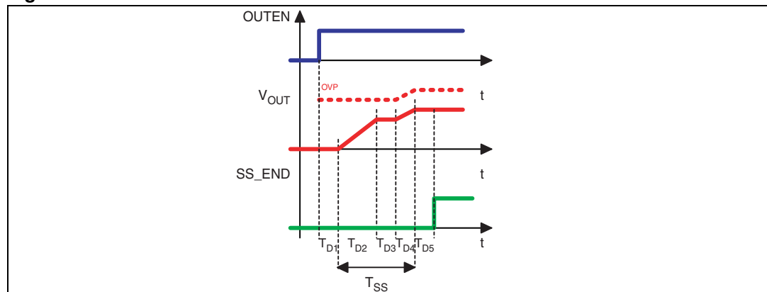
Figure 18. Soft-start
