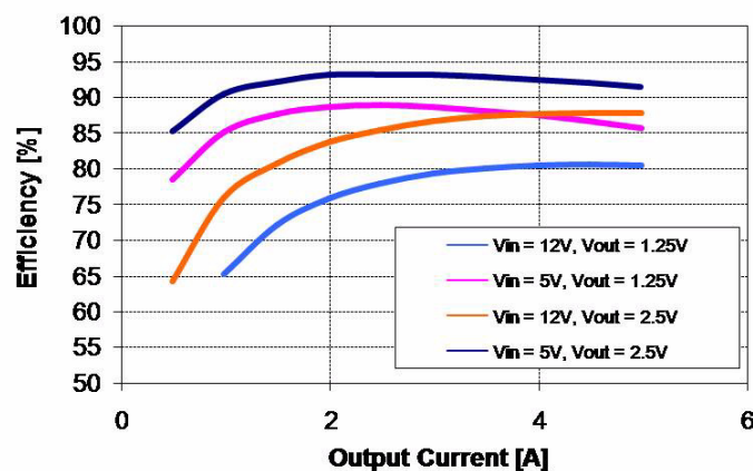
Figure 18. 5 A demonstration board efficiency
