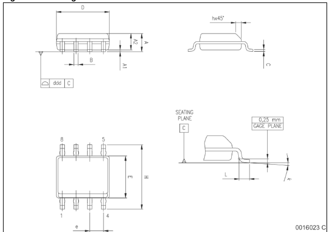
Figure 9. Package dimensions
