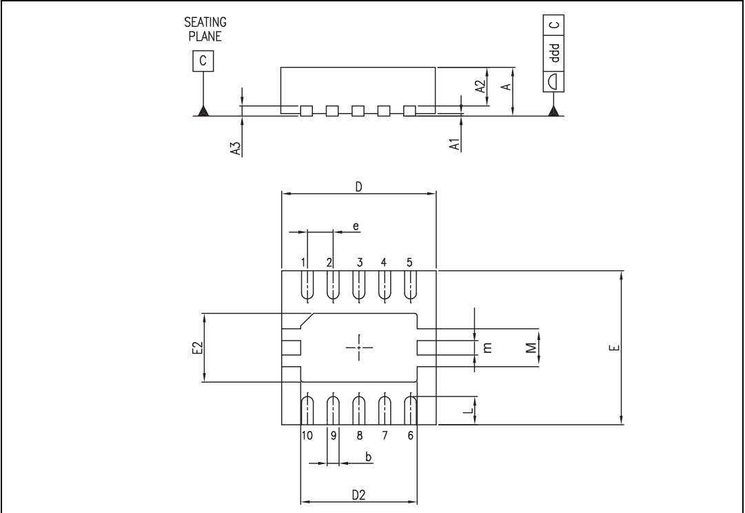
Figure 10. Package dimensions
