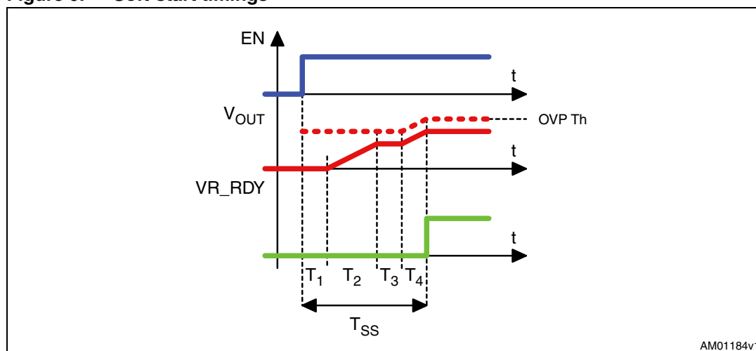
Figure 9. Soft-start timings
