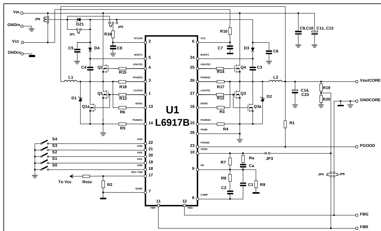
Figure 23. CPU Power Supply Schematic
