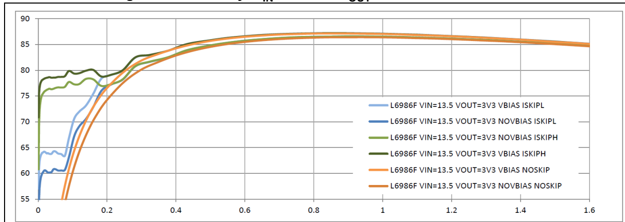
Figure 50. Efficiency: V_{IN} = 13.5\text{ V} - V_{OUT} = 3.3\text{ V} - f_{sw} = 500\text{ kHz}
