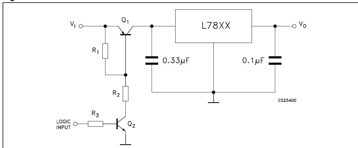
Figure 24. Remote shutdown
