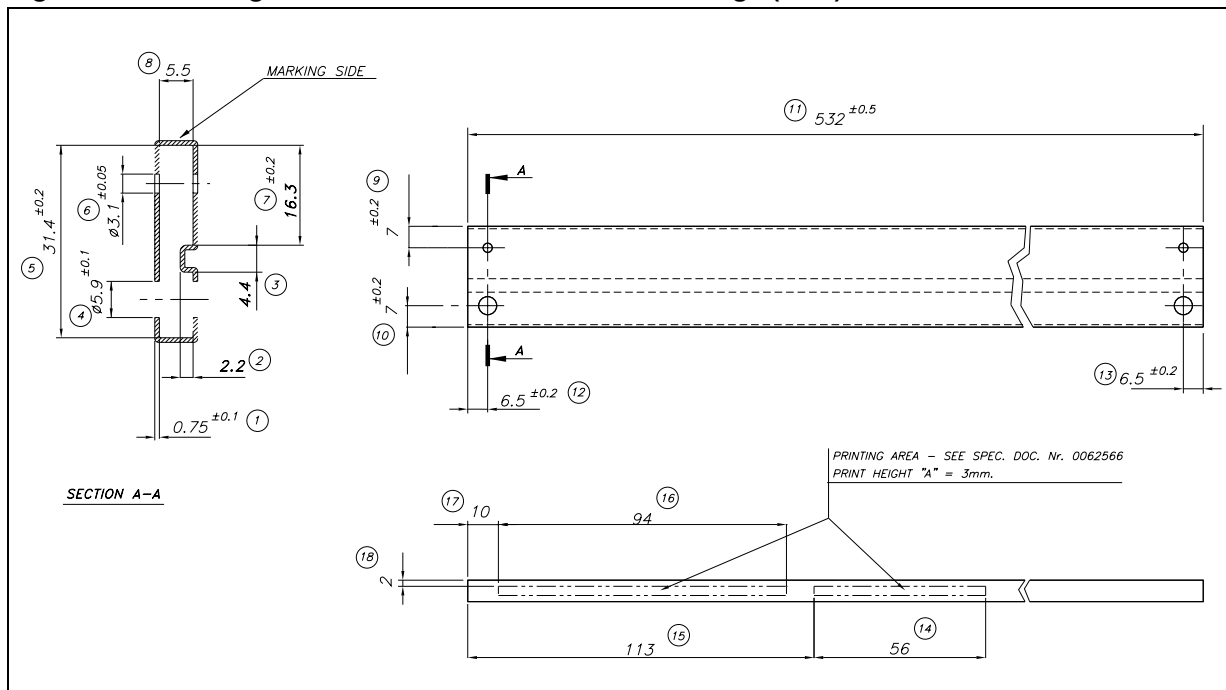
Figure 40. Drawing dimension tube for TO-220 Dual Gauge (mm.)
