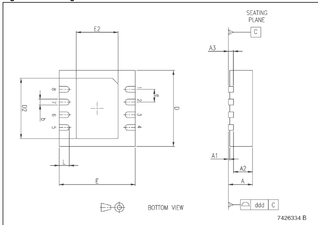
Figure 37. Package dimensions
