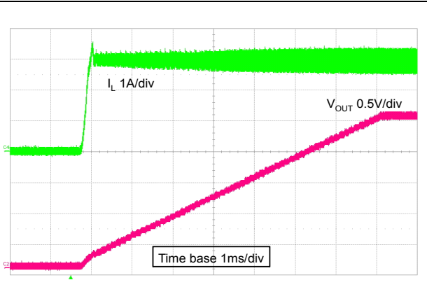
Figure 31. Soft-start
