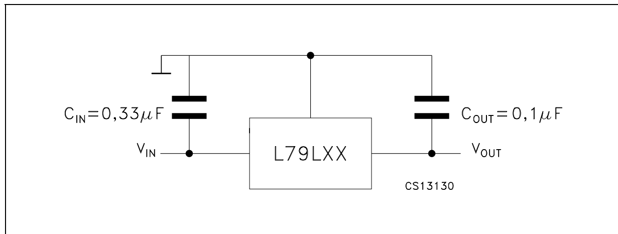
Figure 3: Test Circuits
