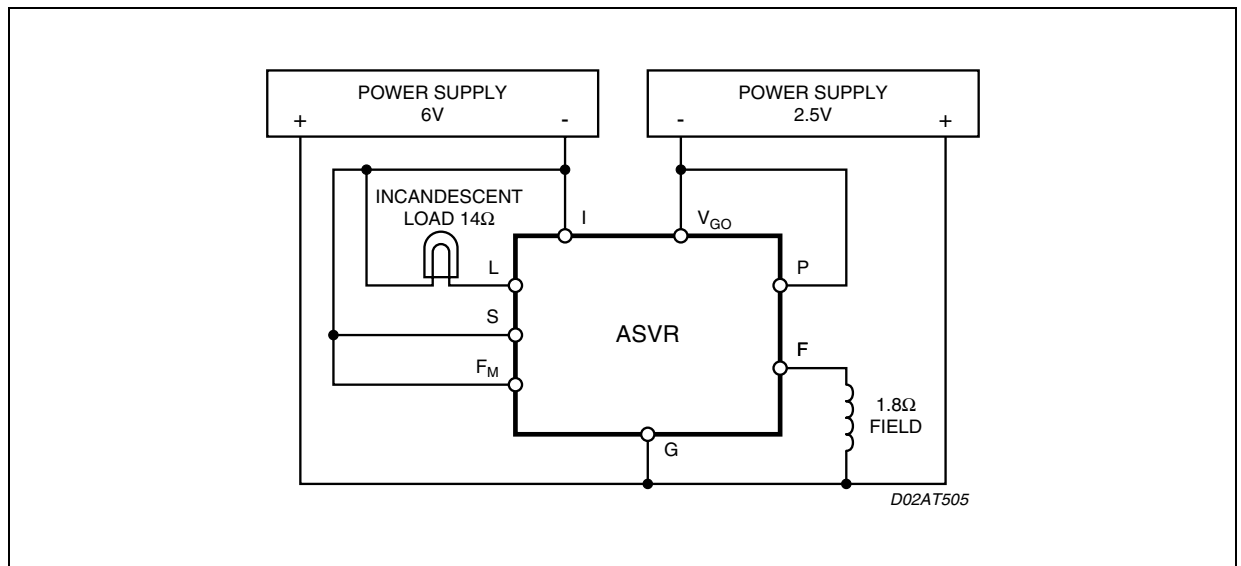
Figure 4. Reverse B+ Test Circuit
