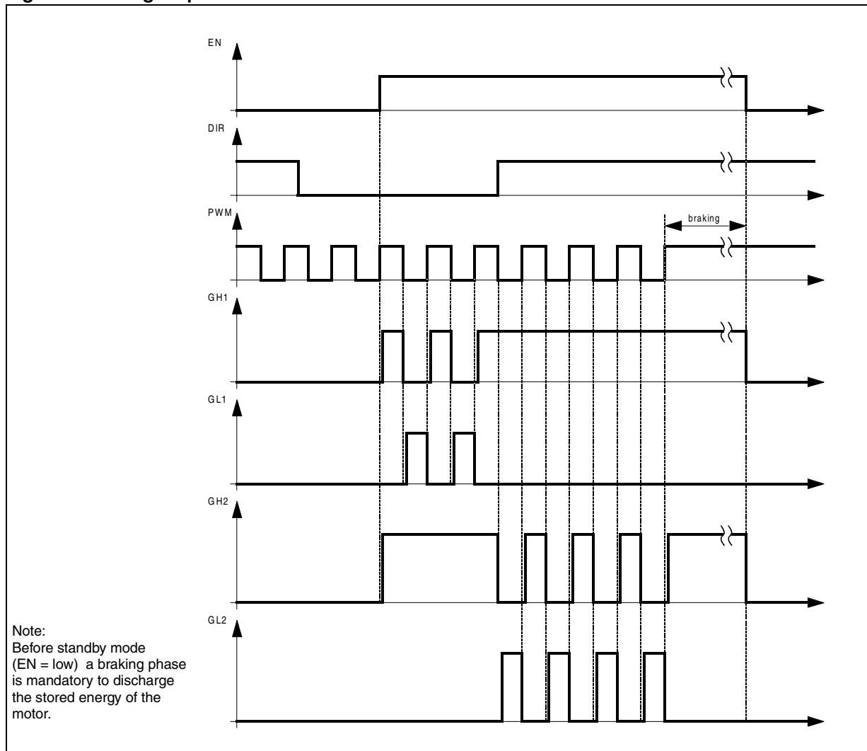
Figure 7. Driving sequence
